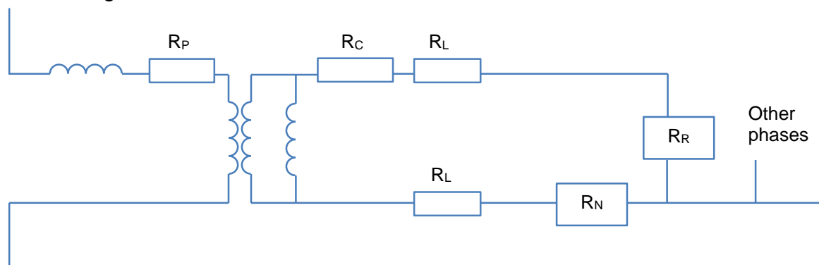
Figure 7. The current transformer scheme with magnetizing reactance and secondary resistance
